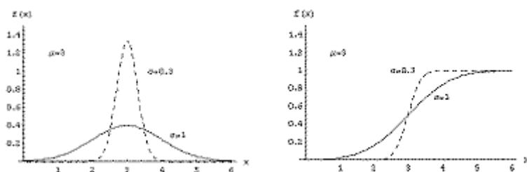
Left: density function ("bell curve"), right: distribution function
