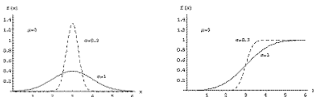
Density function ("bell curve") and distribution function
